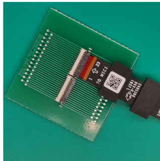
FPC Connector0.5mm
